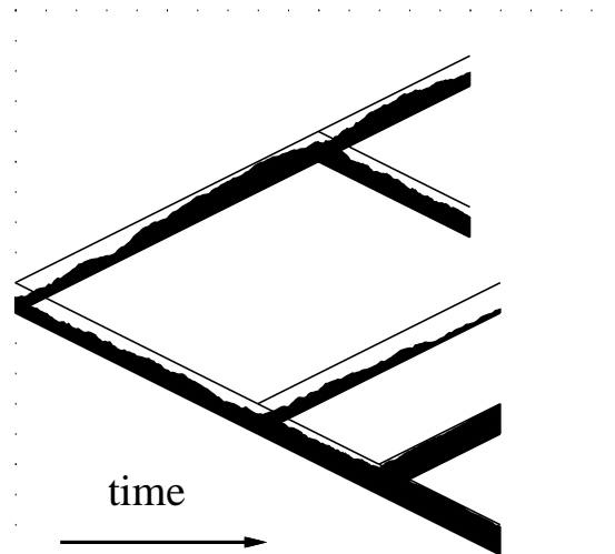
Figure 2: A simulation of a threshold model with one character, evolving by Brownian motion of the liability on a simple 5-species tree. Each lineage is shaded to indicate the proportion of individuals in state 1 (shown by black shading). The upper two species end up with polymorphism, the middle one nearly all with state 0, and the lower ones nearly all with state 1.
