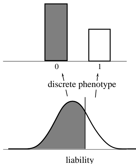
Figure 1: The threshold model of quantitative genetics, showing the continuous distribution of the underlying liability characters, and the resulting discrete distribution of the observed phenotype.
