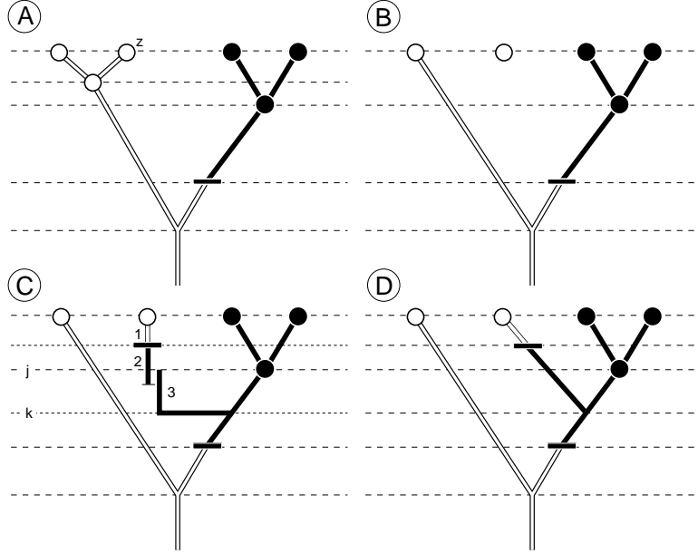
Figure 2: Transition from an old genealogy G_o to a new genealogy G_n . Dotted lines are the times of coalescences or migrations. (A) Genealogy G_o with migration. The black bar marks a migration from the white population to the black or vice versa, z is the node to be picked. (B) Partial genealogy G_p after drawing the coalescent node z at random and dissolving the branch to the next coalescent below. (C) Simulation of the coalescent with migration. One possible outcome with three consecutive steps is shown: (1) using formula 8 a new time interval is drawn and a migration event from white to black is also drawn (formula 9) and the lineage is extended down to that event, (2) a new time interval is drawn: it extends too far back, so the lineage advances down to the time j , (3) a new time interval is drawn with a coalescent event at its bottom end. The process stops at time k . (D) the final configuration G_n .
